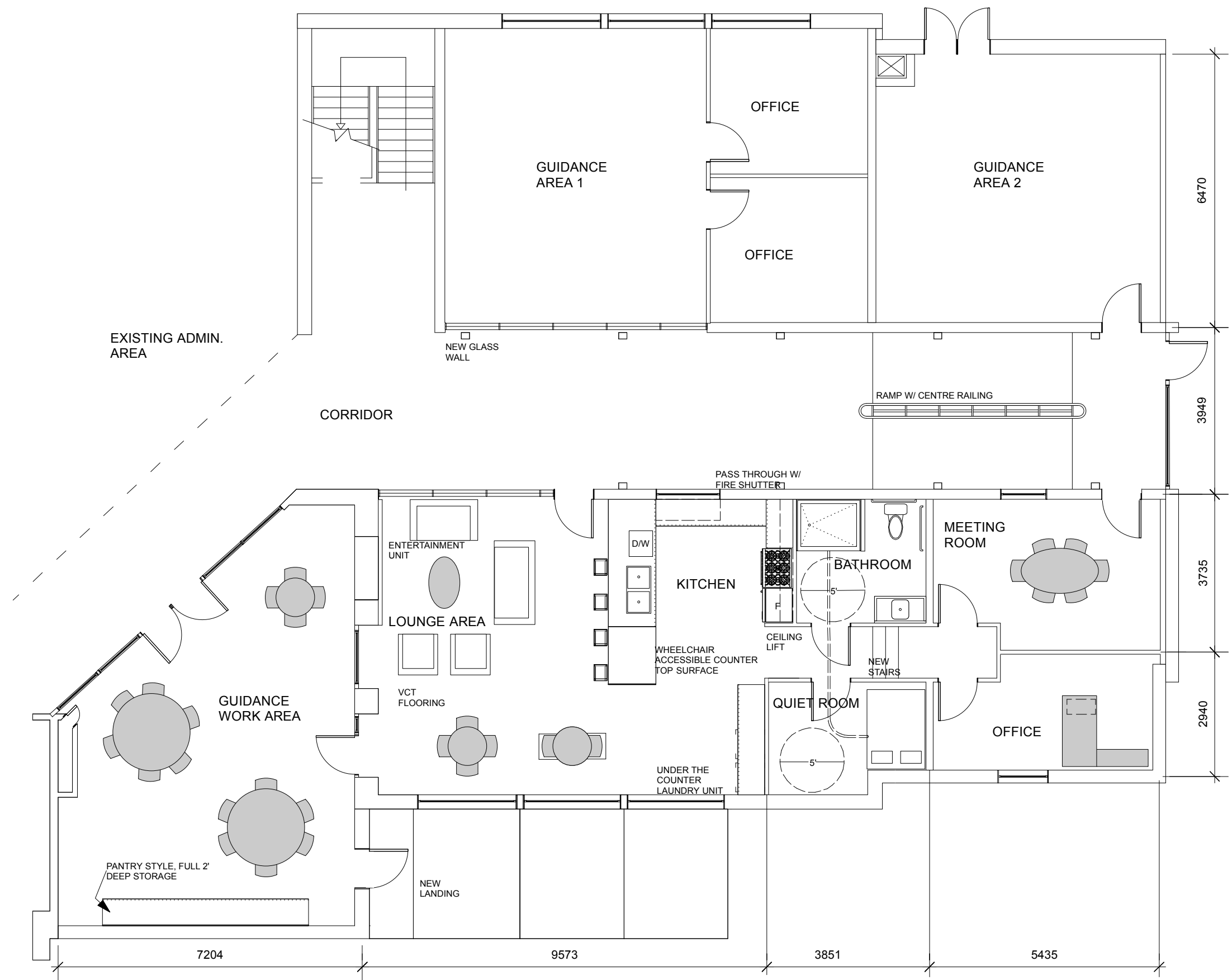
1 PLAN- SPECIAL ED. CENTRE 1:100
